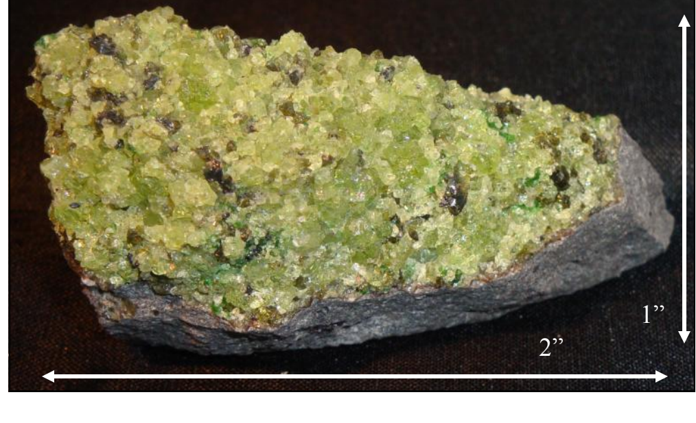
Peridot (green) (Mg, Fe) 2 SiO 4 ) with sphaerulite (?) on basalt Main Old Town, Cottonwood, AZ
